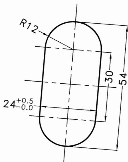
View Z Scale 1:1
