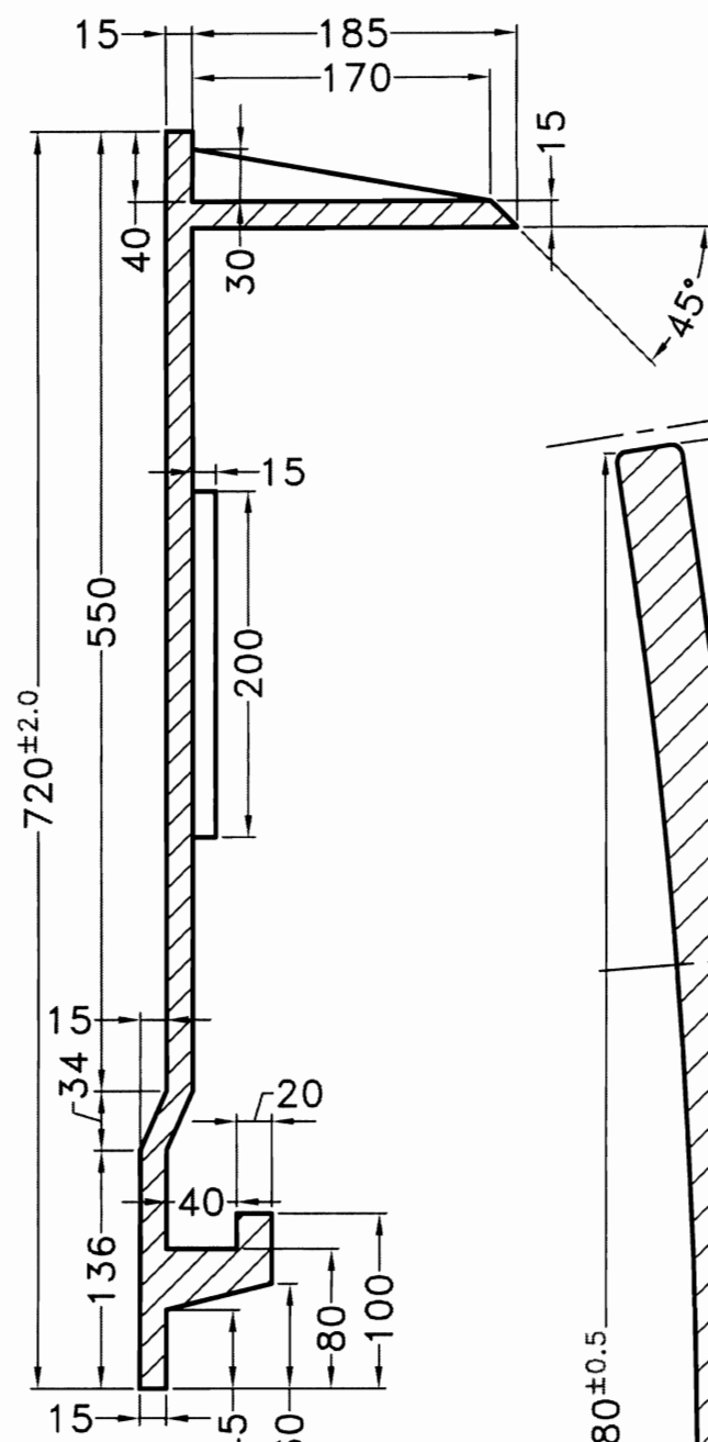
Sec. A-A Scale 1:5
