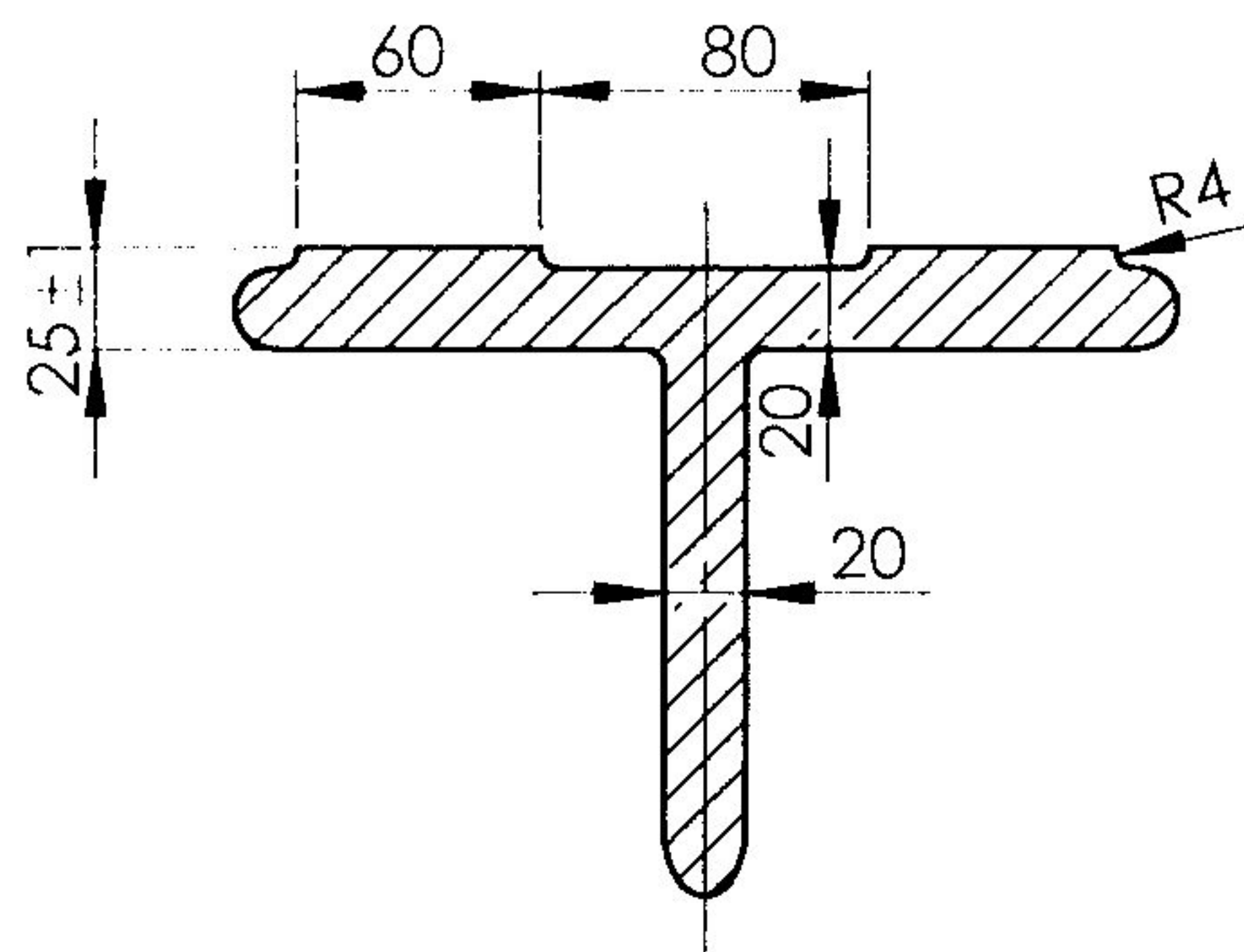
SECTION G-G
