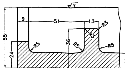
Sec. A-A Scale 1:1
