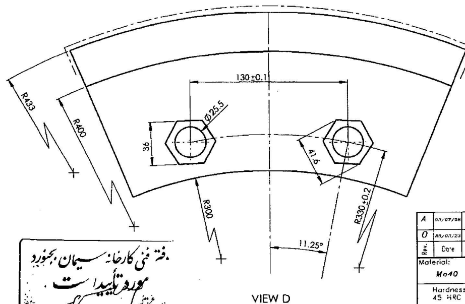
VIEW D
